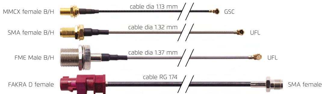
Example of cable assemblies
