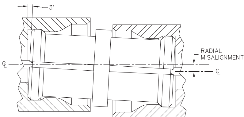
Figure 4 – Radial Misalignment
