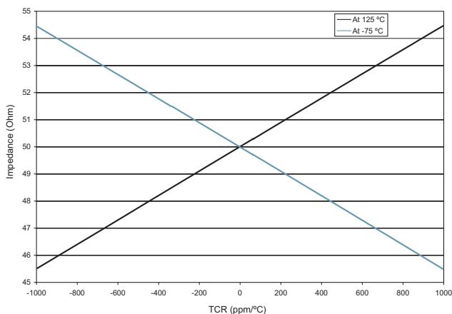
Figure 3. Impedance as a Function of TCR for Two Temperature Extremes, 25 \pm 100 °C.
