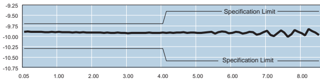
Typical Attenuation Accuracy of a 33-10-34
